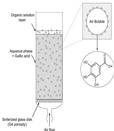
Figure 1: Illustration of the apparatus used in the ATPF. Marked is a typical bubble with the substrate (GA) adsorbed.
