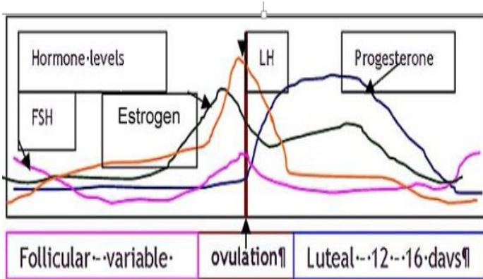
Figure 1: Changes in Hormonal Levels during a Normal Menstrual Cycle.
